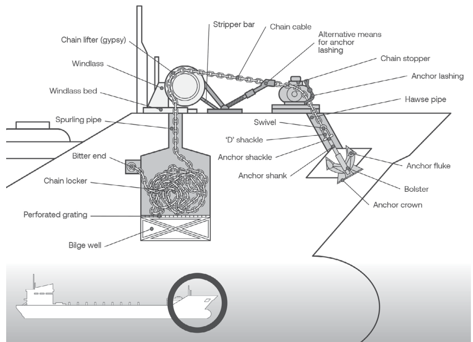
Figure 26.1 Anchoring
